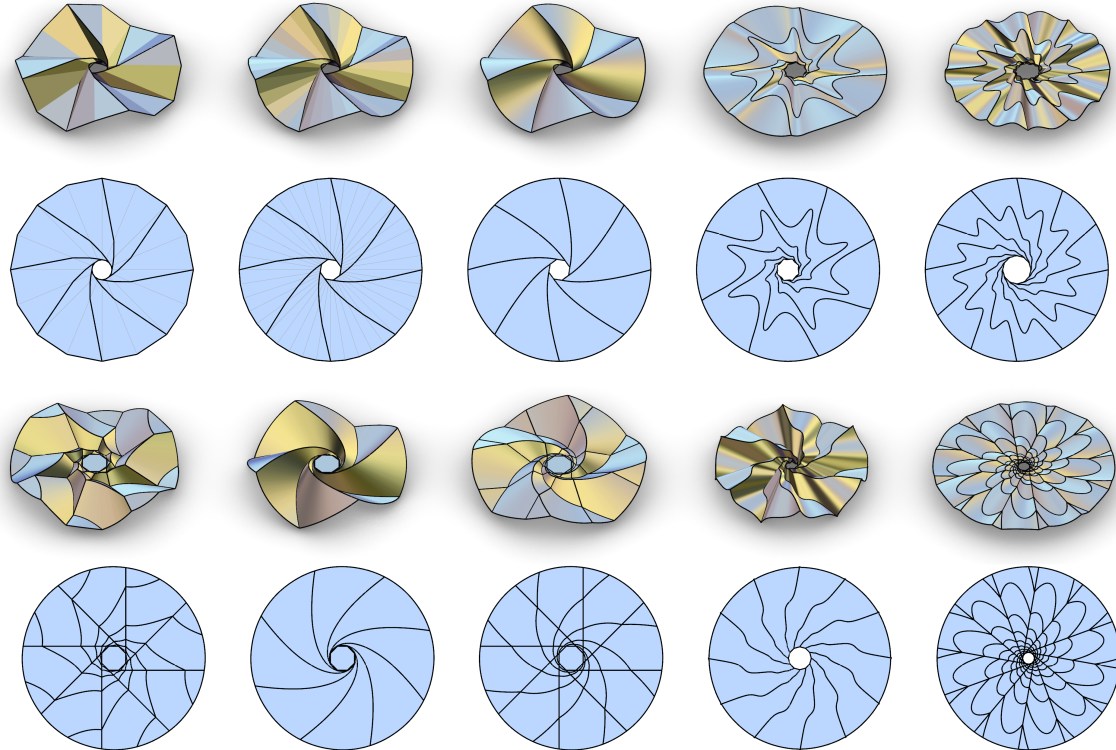
Figure 3: Example designs using our constructions. Top row: Conical spirals. Bottom row: Exploded-vertex spirals with a closed polygonal center when p = 0 .
