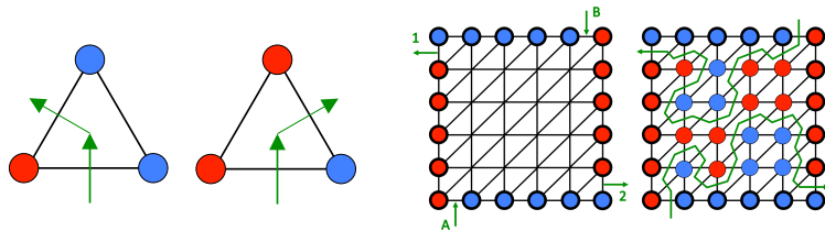
Figure 4 Left: proceeding on a Hex walk through a cell; each step is forced. Right: an empty board (with player-owned edges) has two entries, A and B, and two exits 1 and 2. If the walk entering at A exits through 2 (as shown at far right), then player 1 is the winner; if it exits through 1, then player 2 is the winner.
