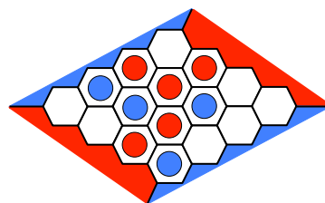
■ Figure 1 A sample Hex position, where Player 1 (red) has won.
