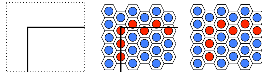
■ Figure 5 Left: A wire occupying part of the space. Middle: The wire, superimposed on the Hex board, with the appropriate tiles turned to red to carry the wire. Right: The wire, represented only as a sequence of red Hex tiles.
