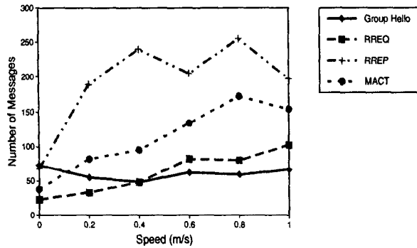
Figure 5: Control Overhead for 50m×50m Multicast Simulations.
